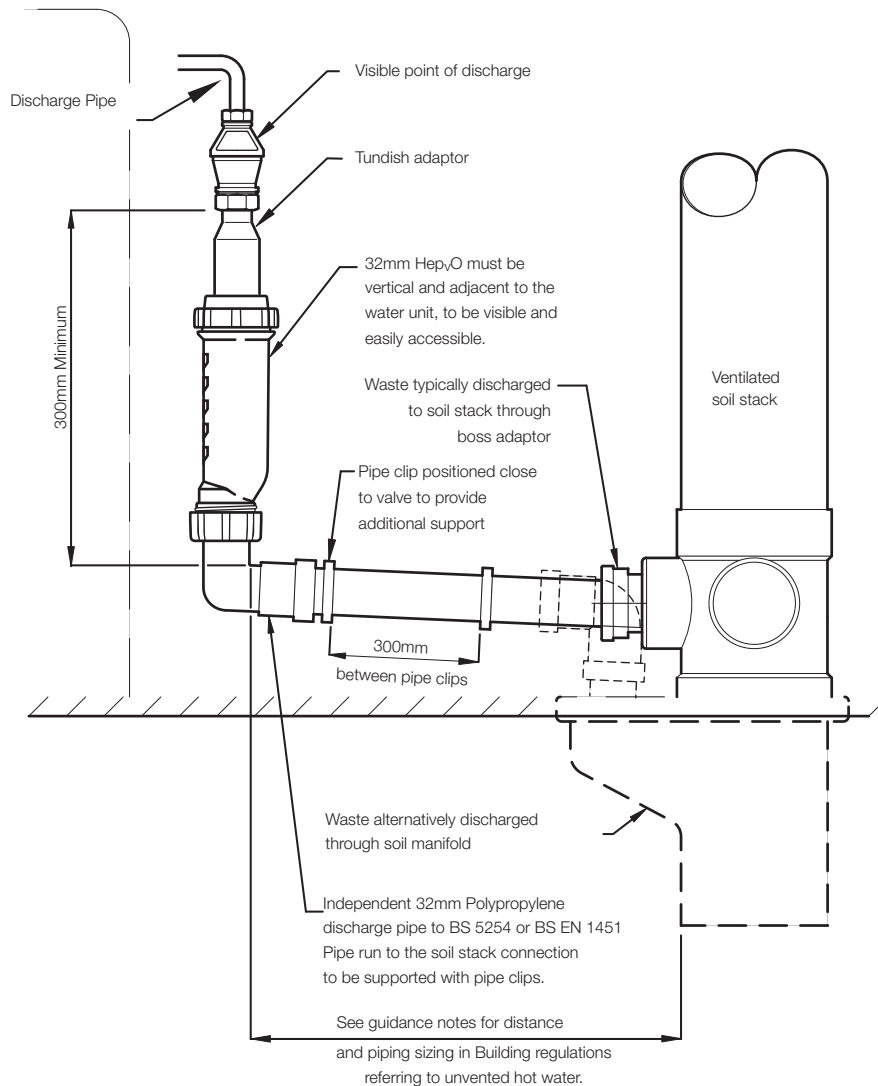
Fig 6 Self-sealing valve when used with a combined temperature and pressure relief valve for unvented hot water storage system.
