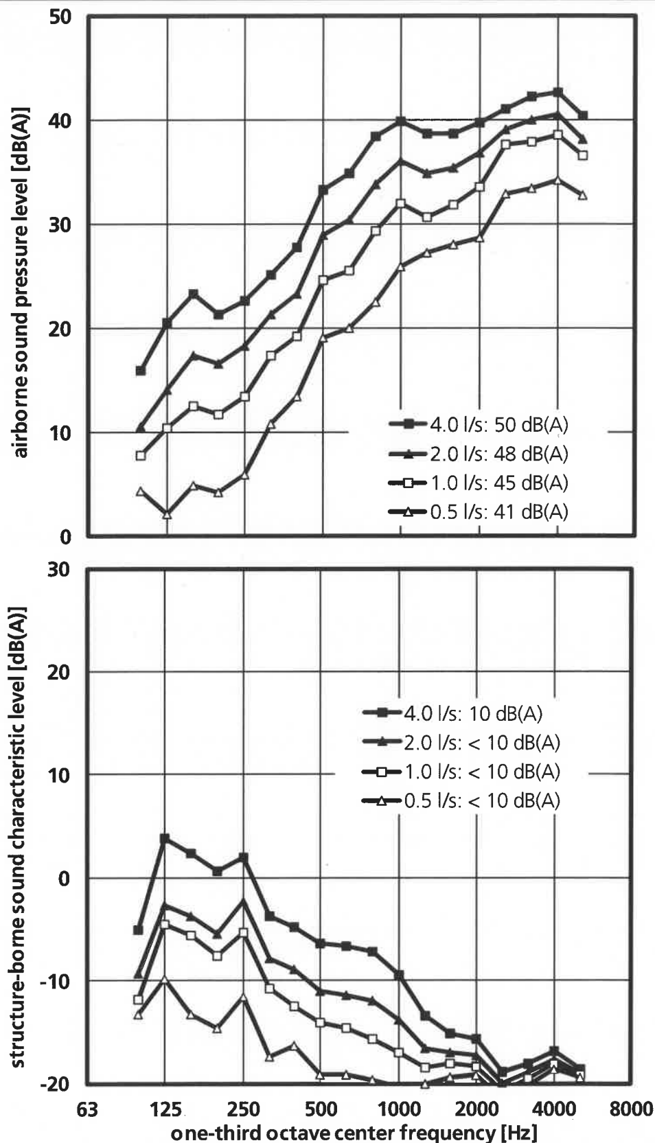
Frequency spectrum of the airborne sound pressure level L_{p,A} (above) and structure-borne sound characteristic level L_{sc,A} (below) measured at various flow rates according to EN 14366.
