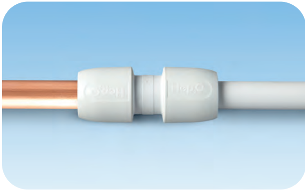
Example 1: Copper Pipe with Hep20 Fitting (Including demounting & re-use)
