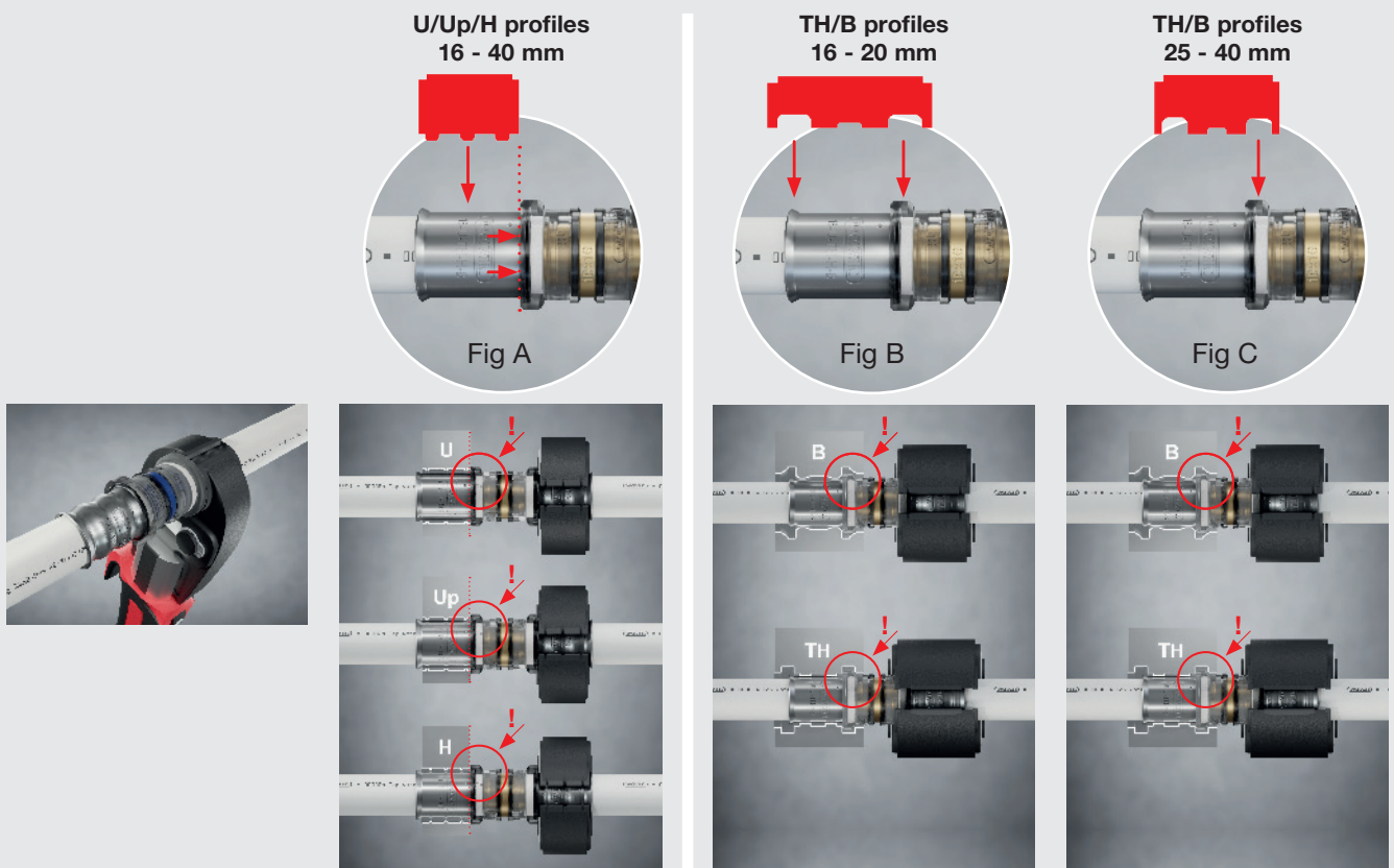
Fig. 25: Positioning the pressing jaws on the fitting with Tigris K5 and Tigris M5.
