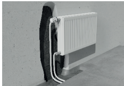
Fig. 47: Radiator installation examples with “Eurocone” screw connection.
