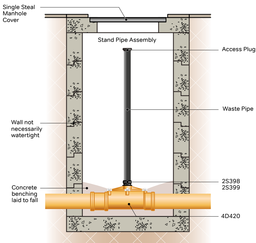
Figure 24: Sealed Access Manhole and standpipe
