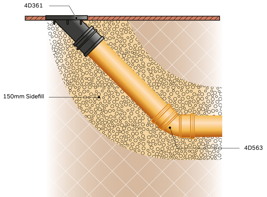
Figure 25: Rodding Eye – head of drain access
