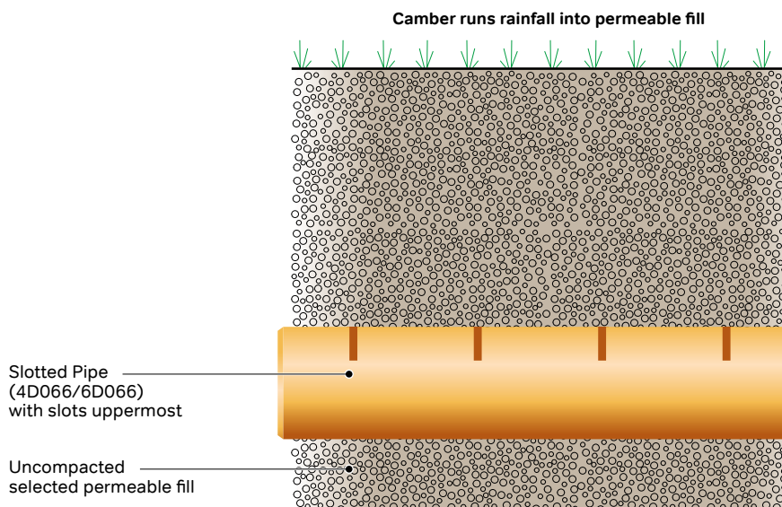
Figure 37: French Drain
