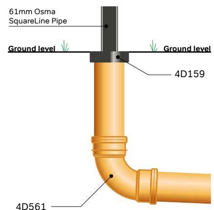
Figure 21: Connection of SquareLine Rainwater Pipes
