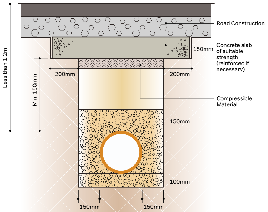
Figure 8: Pipe Protection – concrete slab
