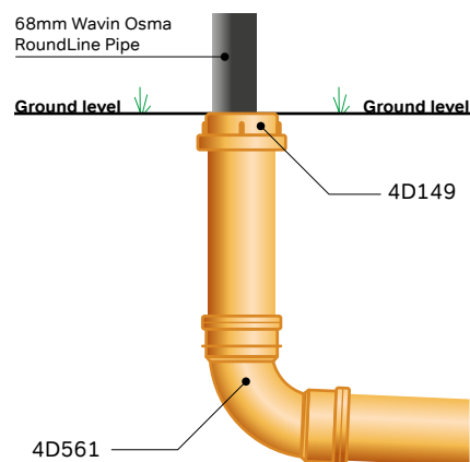
Figure 18: Connection of RoundLine rainwater pipe to Wavin OsmaDrain 110mm socket
