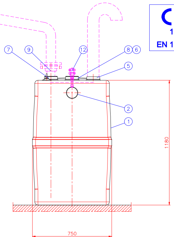
Indoor installation model (On the floor)
