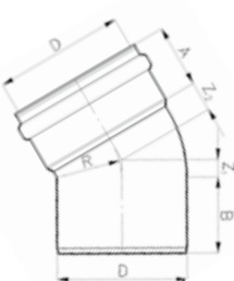
Solidwall PVC SN12 - Koleno 30°
