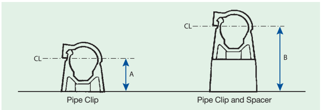
Figure 35: Pipe fixing centres
