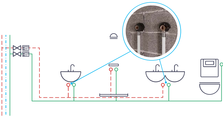
Fig. 40: Single Tee installation.
