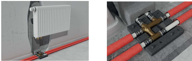
Fig. 46: Radiator installation examples with crossfitting block.
