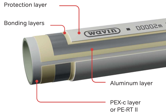
Fig. 1: Multilayer composite pipe structure.
