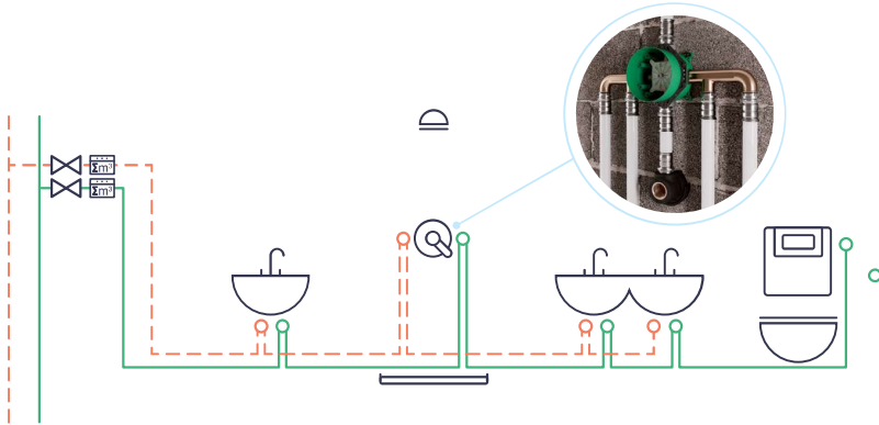
Fig. 41: In series installation.
