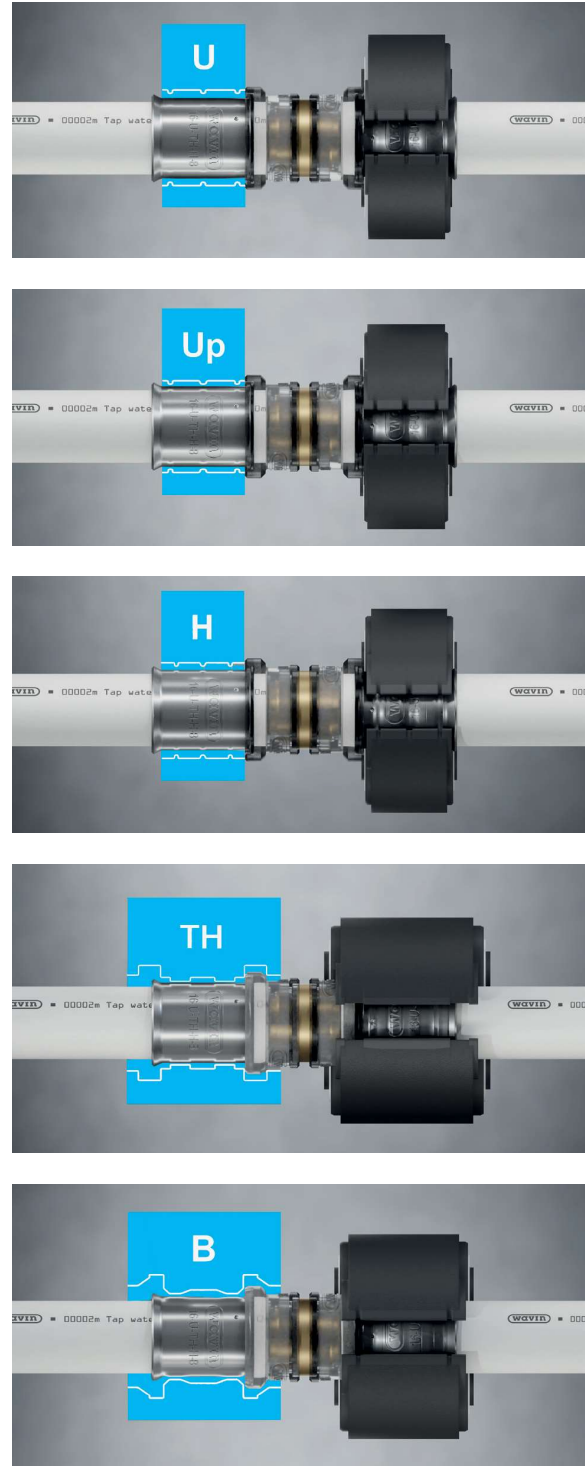
Fig. 48: Released pressing profiles for Tigris K5/M5.
