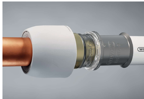
Fig. 29: Push-fit transition to copper for Tigris M5.
