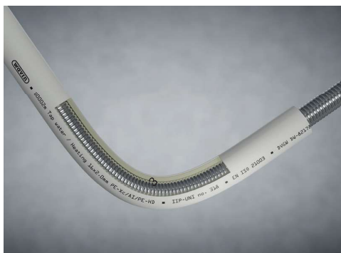
Fig. 24: Bending the pipe with a bending spring.
