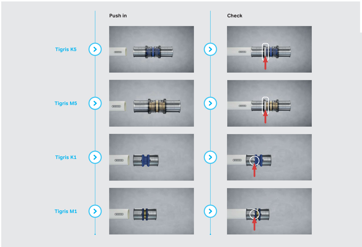
Fig. 22: Checking the correct pipe insertion.
