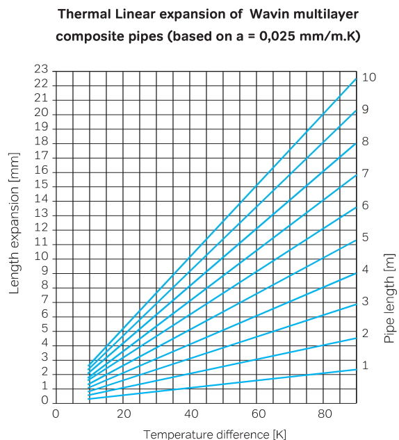
Fig. 36: Thermal Linear expansion.
