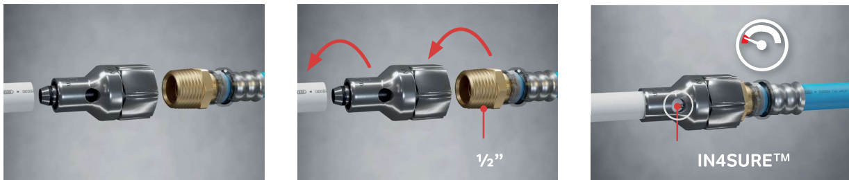
Fig. 35: Pressure check with coupler: 16 mm - 20 mm - 25 mm.
