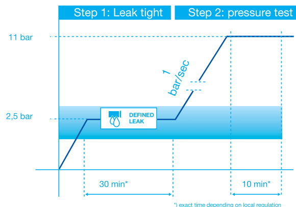
Fig. 33: Pressure test protocol when testing with water.
