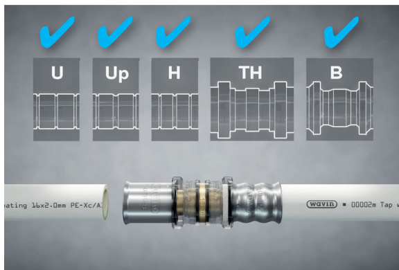
Fig. 11: MULTI JAW.
