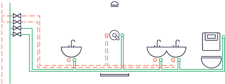
Fig. 42: Loop installation.
