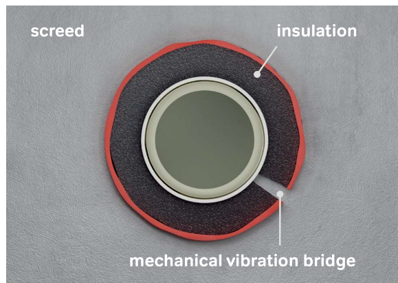
Fig 39: Mechanical vibration transmission through defective pipe insulation.
