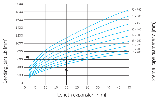
Fig. 37: Bending joint classification of Wavin multilayer composite pipes.
