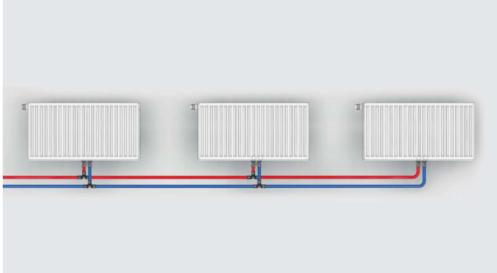
Fig. 44: Double pipe radiator heating.
