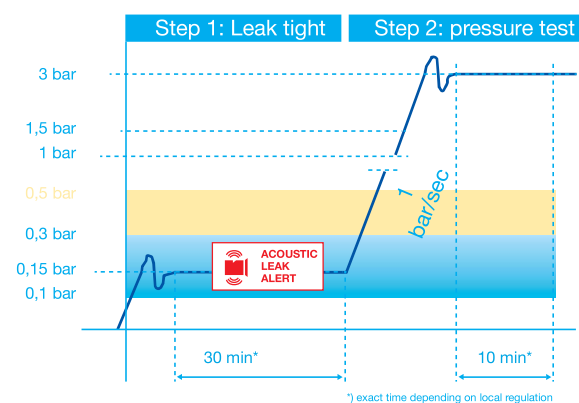
Fig. 34: Pressure test protocol when testing with air.
