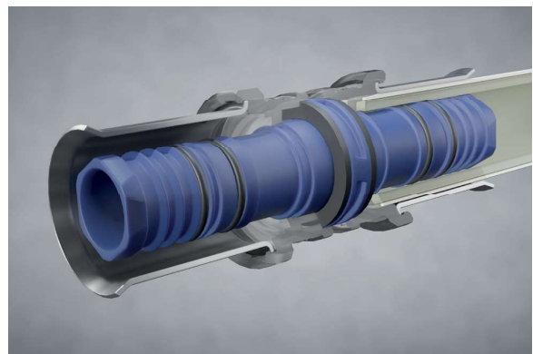
Fig. 12: EASYFIT. Pipe insertion without calibration.
