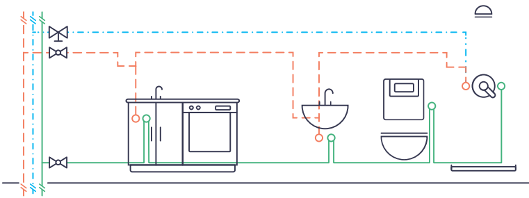
Fig. 43: Loop installation with circulation connection.
