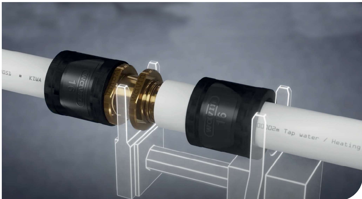
Fig. 5: Ultimate-Flow Tigris MX connection.
