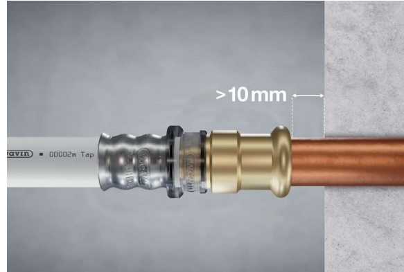
Fig. 28: Minimum distance between fitting and wall.
