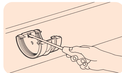
Figure 26: Fixing Gutter Jointing Bracket (OT005)
