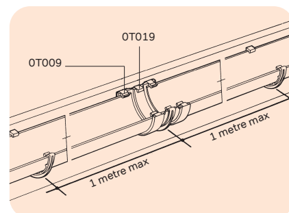
Figure 27: Installation of RoundLine Gutter Union
