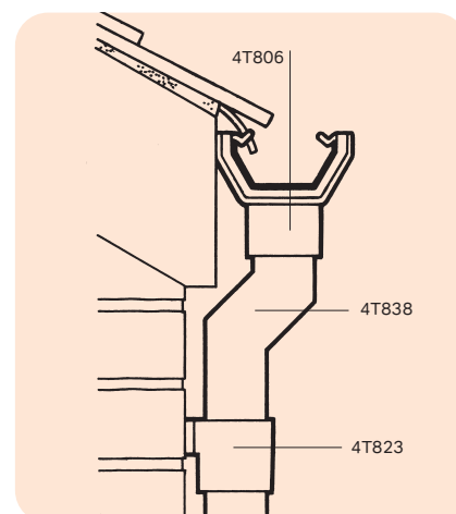
Figure 11: SquareLine shallow offset
