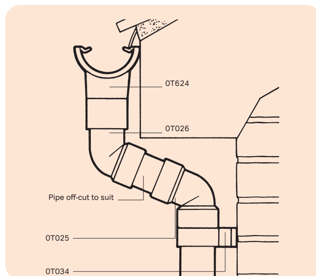
Figure 47: Offset on deep fascia
