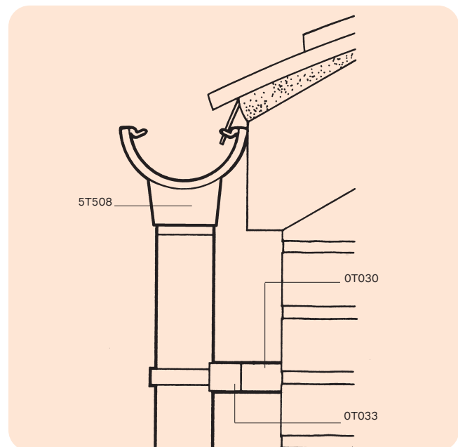
Figure 44: Application of Pipe Bracket Spacer
