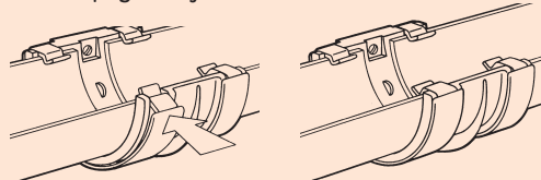
'Flexiclip' gutter joint.
