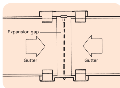
Figure 5: Allowance for thermal movement
