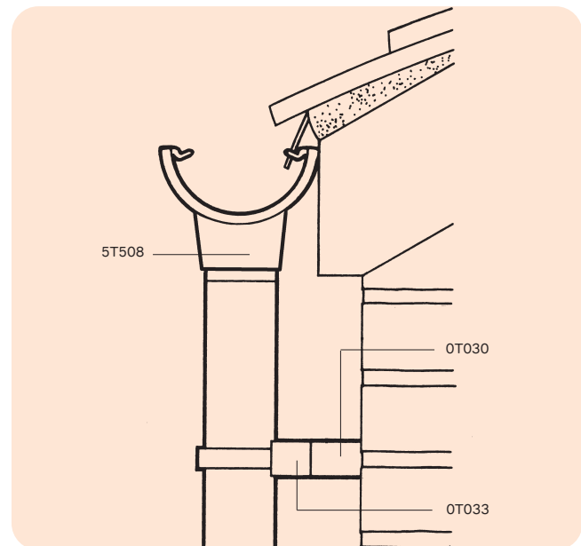
Figure 8: Application of Pipe Bracket Spacer
