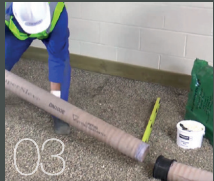
03 Push into previously laid SuperSleve pipe
