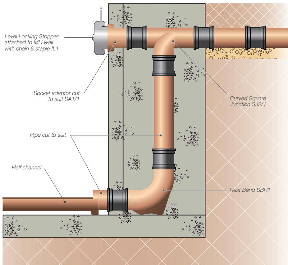
Fig. 39 – Backdrop connections
