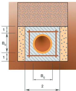
c. Reinforced concrete surround. Bedding factor 4.8 (4 × 1% steel). Reference: TRRL Simplified tables [2]
