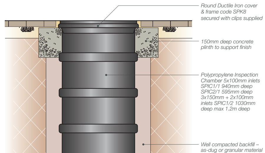
Fig. 29 – Installation detail – domestic paths/patios
