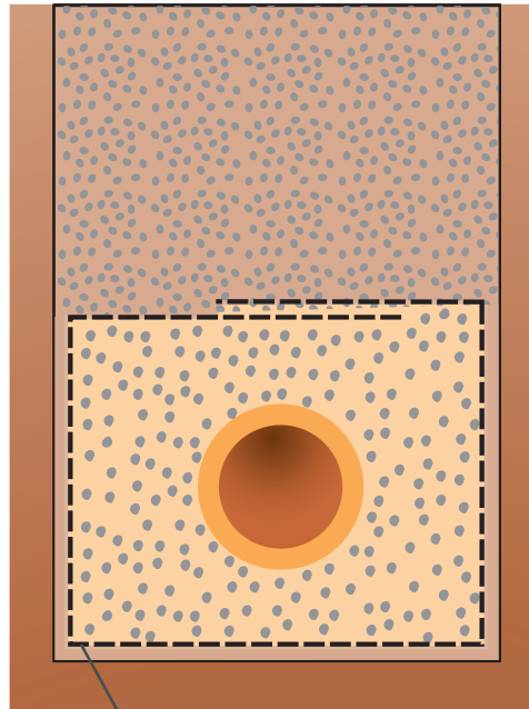
Fig. 7 – Use of Geotextile material around pipe bedding in waterlogged ground
