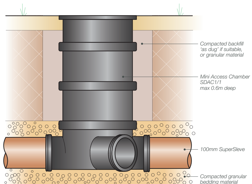
Fig. 26 – Installation detail – domestic gardens
