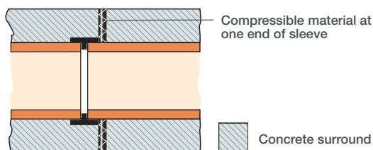
Sleeve jointed pipes in a concrete surround
