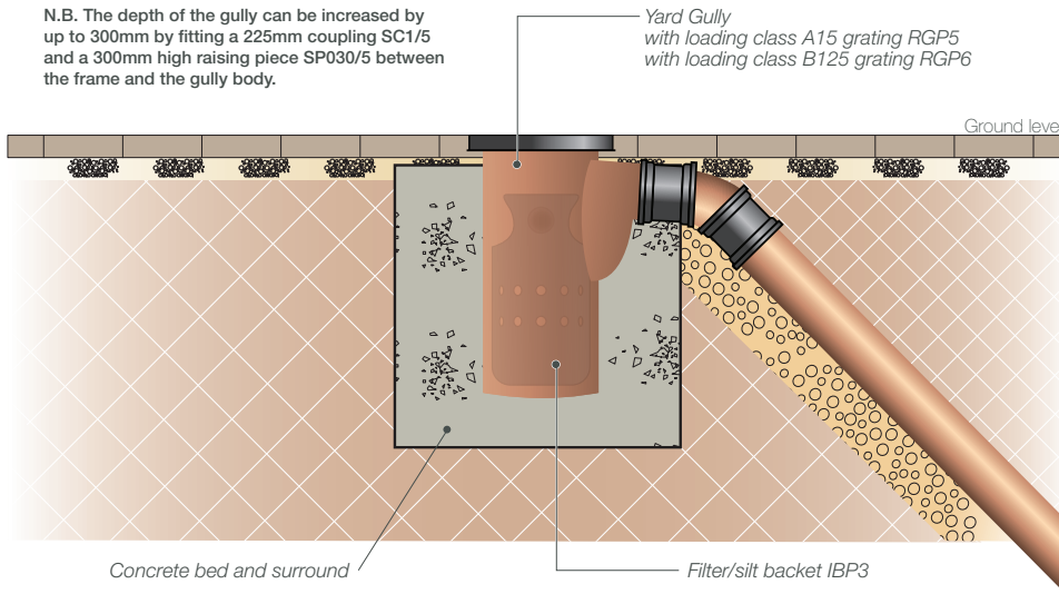
Fig. 24 – Yard Gully
