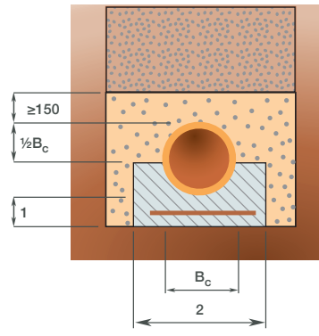
b. Reinforced concrete bed. Bedding factor 3.4 (0.4% steel)
