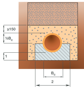
d. Unreinforced concrete bed. Bedding factor 2.6
