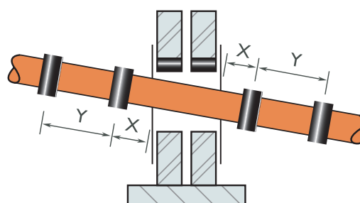
b. Pipe through lintelled opening
