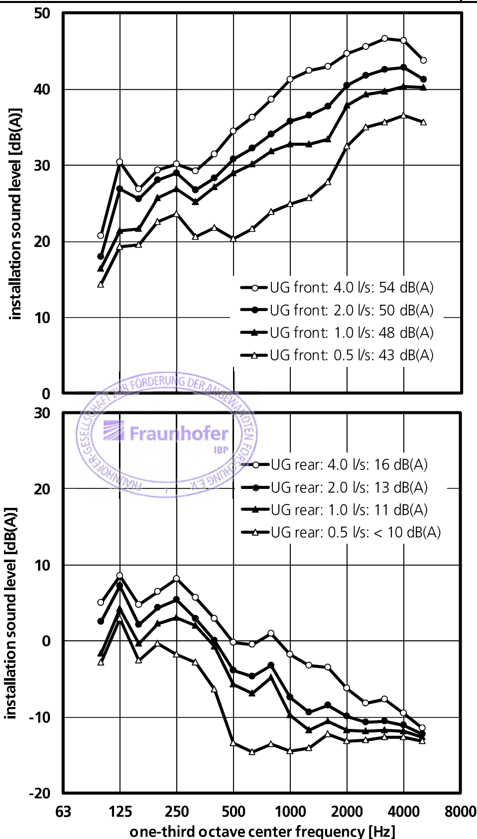
Frequency spectrum of the installation sound level L_{A,Feq,n} measured at various flow rates in the test rooms UG front (above) and UG rear (below). The installation sound levels L_{A,Feq,n} in dB(A) following DIN 4109, for the reproduced frequency range from 100 to 5000 Hz, are represented in the legend.
