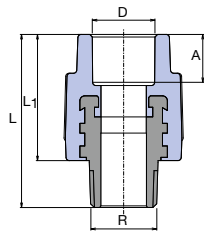
Reducing Sleeve with Metal Male Thread
