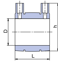
Electrofusion Coupling S 5 / SDR 11
