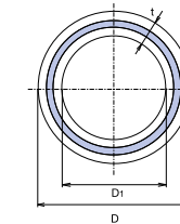
Wavin Ekoplastik PP-RCT Fiber Basalt Clima pipe 20 - 25 mm – S 4 / SDR 9 / PN 22 (calculation) 32 - 125 mm – S 5 / SDR 11 / PN 18 (calculation)
