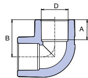
Elbow 90°
