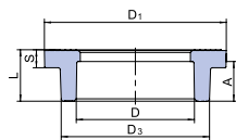
Flange Adaptor
