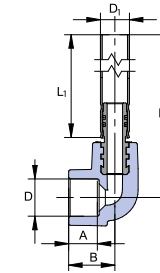
Radiator Connector Elbow 90°
