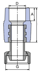
Metal Reducer Cap Nut - Eurokonus
