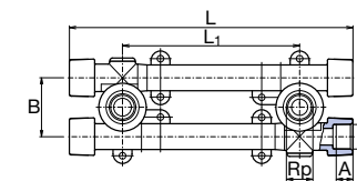
Wall Mounting Group with Tap Connectors for Gypsum Wall
