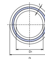
Wavin Ekoplastik PP-RCT Basalt Clima pipe S 5 / SDR 11
