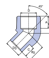
Elbow 45° Internal / External
