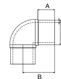
Elbow 90° PP-RCT (Butt Fusion) S 5 / SDR 11
