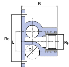
Ending Wall Elbow Right
