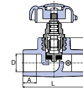
Straight - Way Valve with Drain Valve
