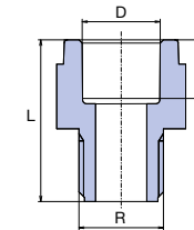
All-Plastic Reducer Male Thread
