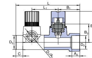
Manifold with Regulation 2 Circuits PP-RCT
