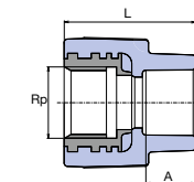
Reducing Sleeve with Metal Female Thread
