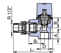
Radiator Valve Angle with Thermostat
