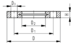
Flange PP-Glass Fiber Reinforced PN16
