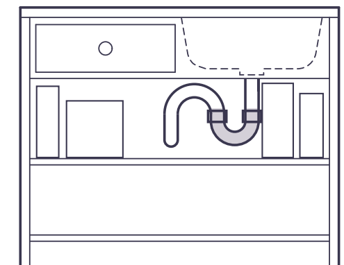
Sink cupboard with water seal trap
