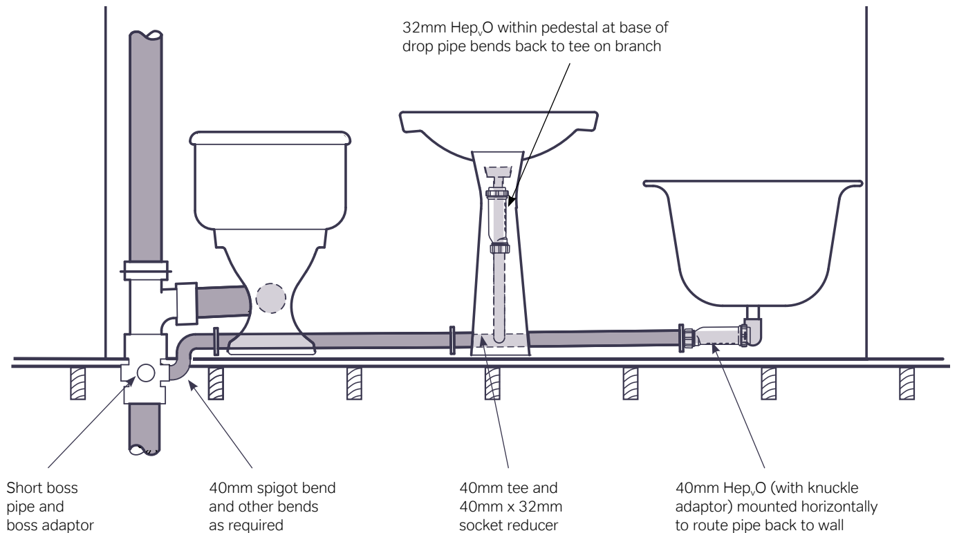
Fig 11. Hep v O installation in a typical bathroom
