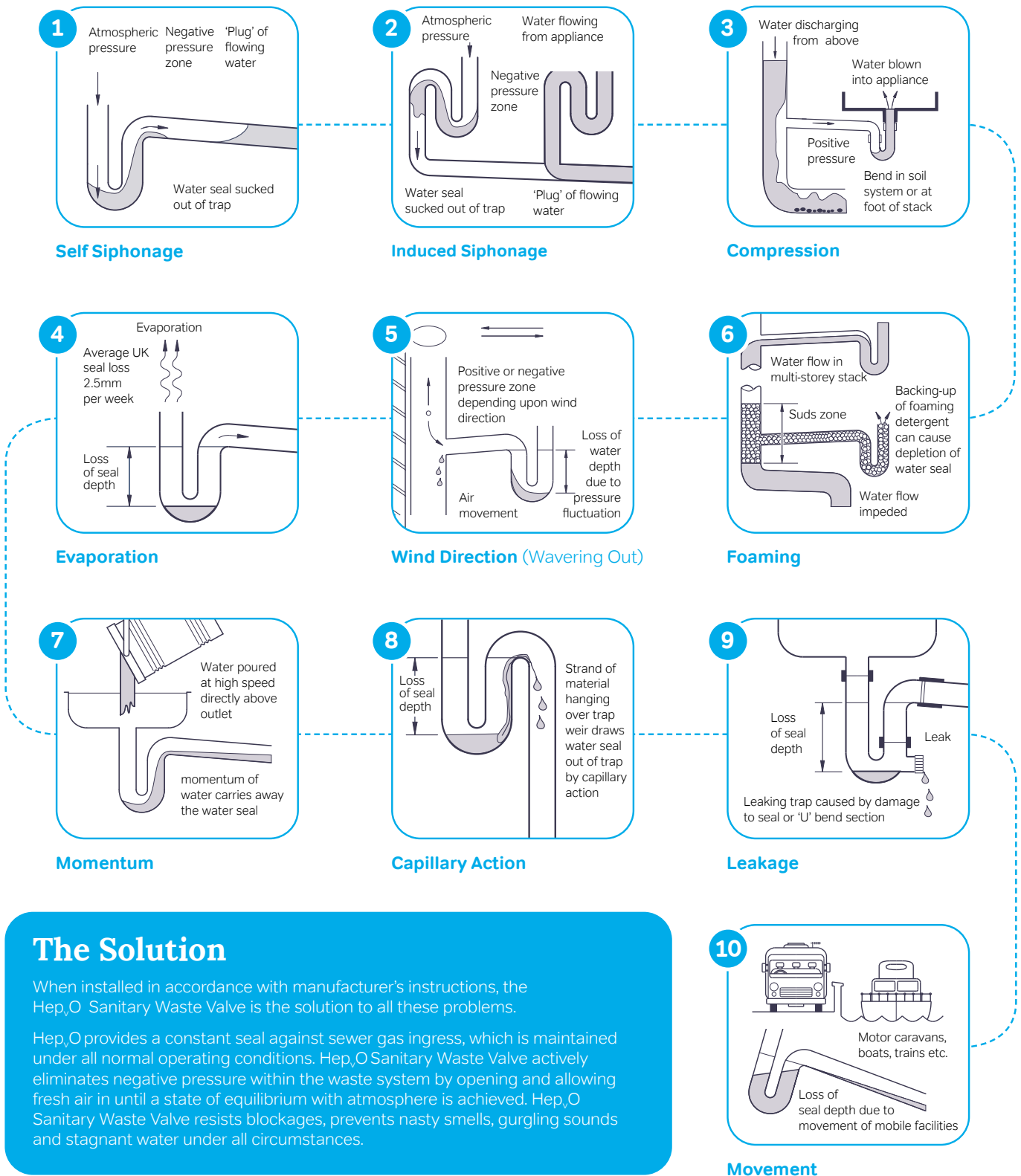
Fig 2. Ten potential reasons for trap failure
