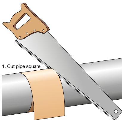
Figure 41: Pipe preparation
