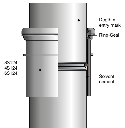
Figure 42: Ring-seal joint
