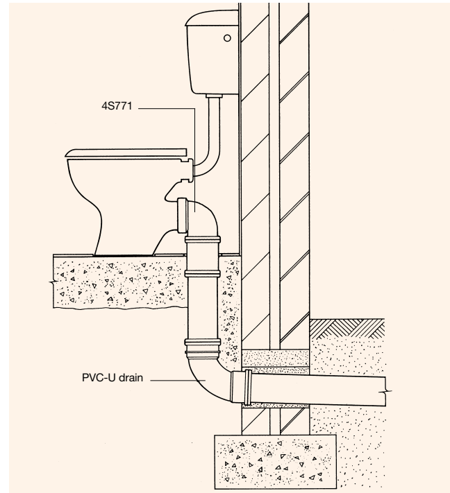
Figure 24: Connection to ground floor WC
