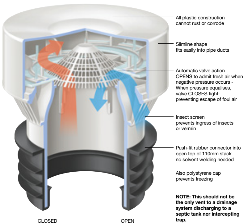
Figure 32: Valve operation
