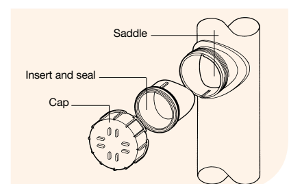
Figure 7: Access Saddle (4S275)
