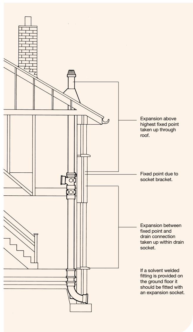
Figure 5: Thermal movement requirements for a Solvent Weld Soil system
