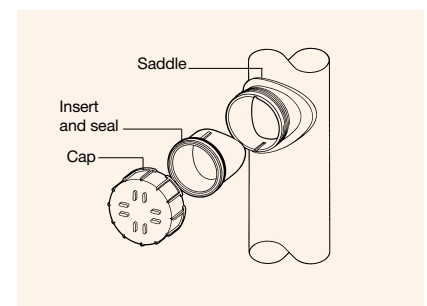
Figure 51: Access Saddle
