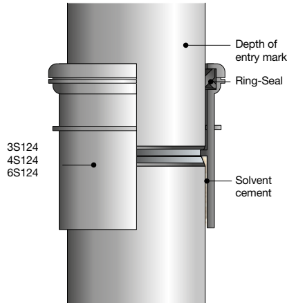
Figure 43: Solvent cement joint
