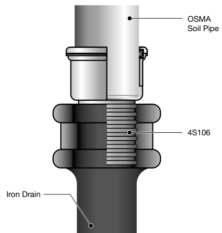
Figure 49: Cast iron drain socket
