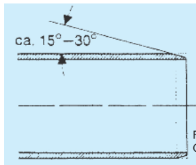
Figure 3: Chamfering in pipe ends
