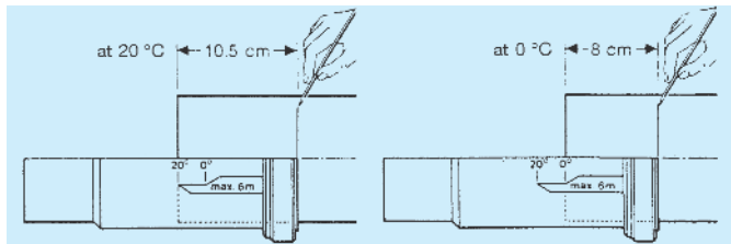
Figure 5: Insertion length as a function of installation temperature
