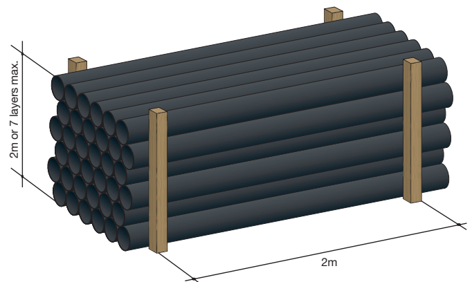
Figure 16: Pipes stored on timber supporting frame
