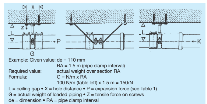
Figure 6: Examples of anchor point attachment
