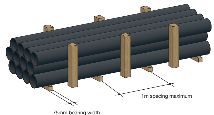
Figure 16: Pipes stored on timber supporting frame
