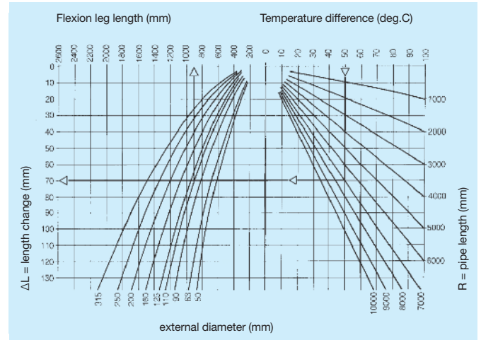
Figure 2: Calculation of flexion leg length
