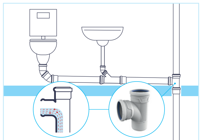
Figure 35: Representation of streamlined moulded parts
