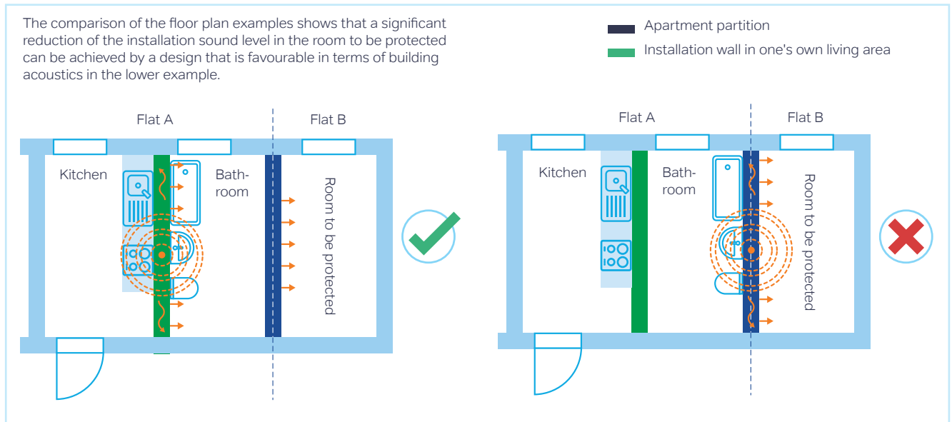
Figure 22: A floor plan favourable from the point of view of building acoustics
