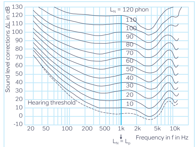
Figure 4: Connection between subjectively perceived sound volume L_N and objectively measurable sound pressure level L_p . L_N and L_p only match at the frequency f = 1000 Hz.
