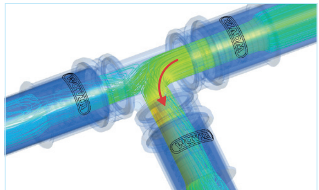
Figure 34: Flow conditions in a tee
