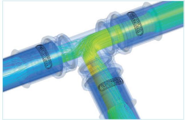
Figure 10: Flow conditions in a tee
