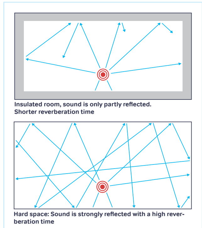
Figure 8: Sound reflection
