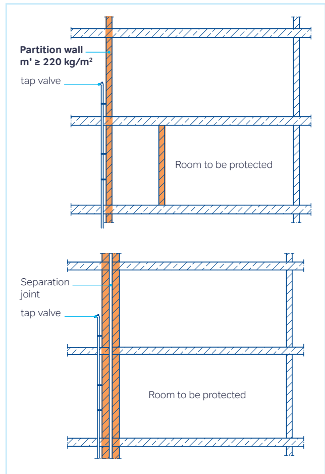
Figure 28: Arrangement of fittings of fitting group II
