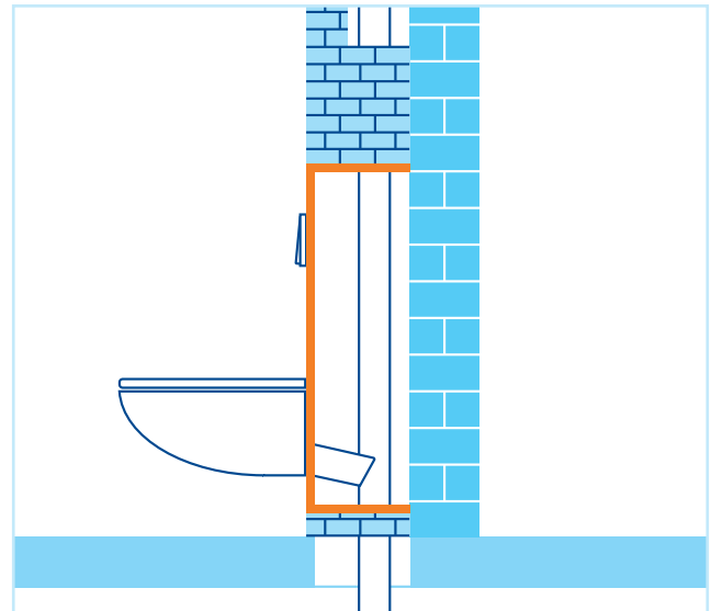
Figure 30: Walling off in wet construction in front of solid wall (based on source 8)
