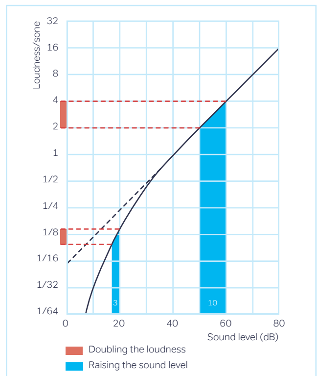
Figure 6: Subjective perception of sound volume according to Zwicker
