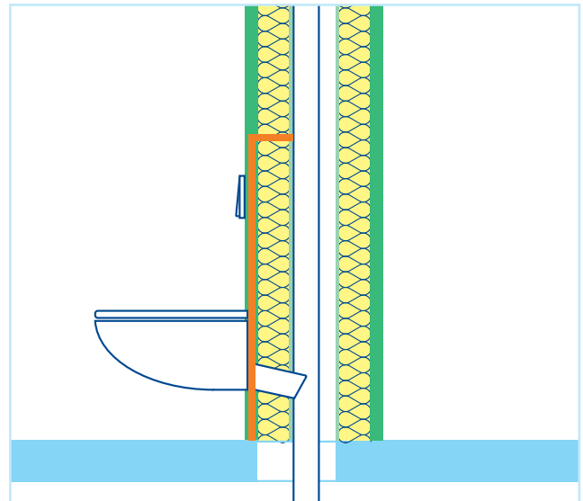
Figure 33: In-wall installation (based on source 8)
