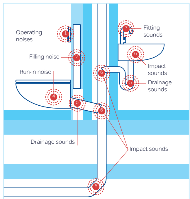
Figure 18: Noise sources in drinking water and wastewater installations
