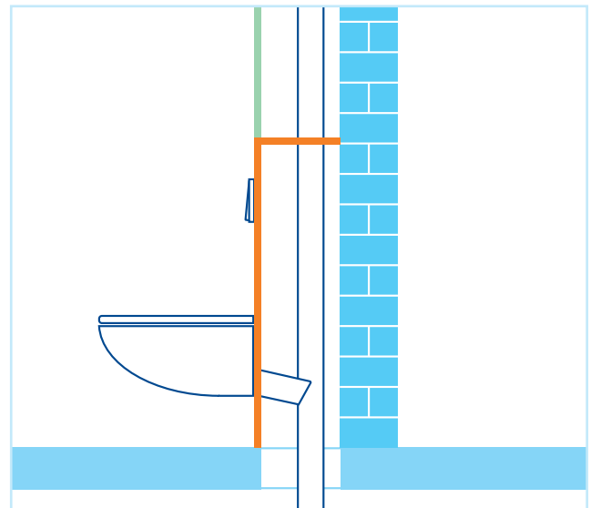
Figure 31: Drywall curtain wall in front of solid wall (based on source 8)
