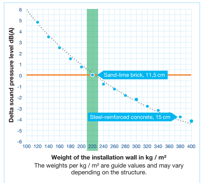
Figure 23: Illustration of the change in sound pressure level in the adjacent room as a function of different wall materials from Wavin SoundCheck.
