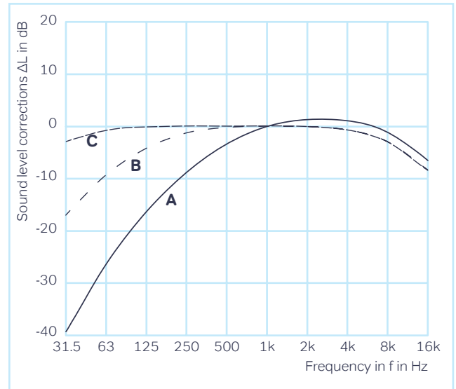
Figure 2: Sound pressure level correction ΔL according to DIN EN ISO 16032 (or the withdrawn DIN EN 60651) for ratings A, B, and C
