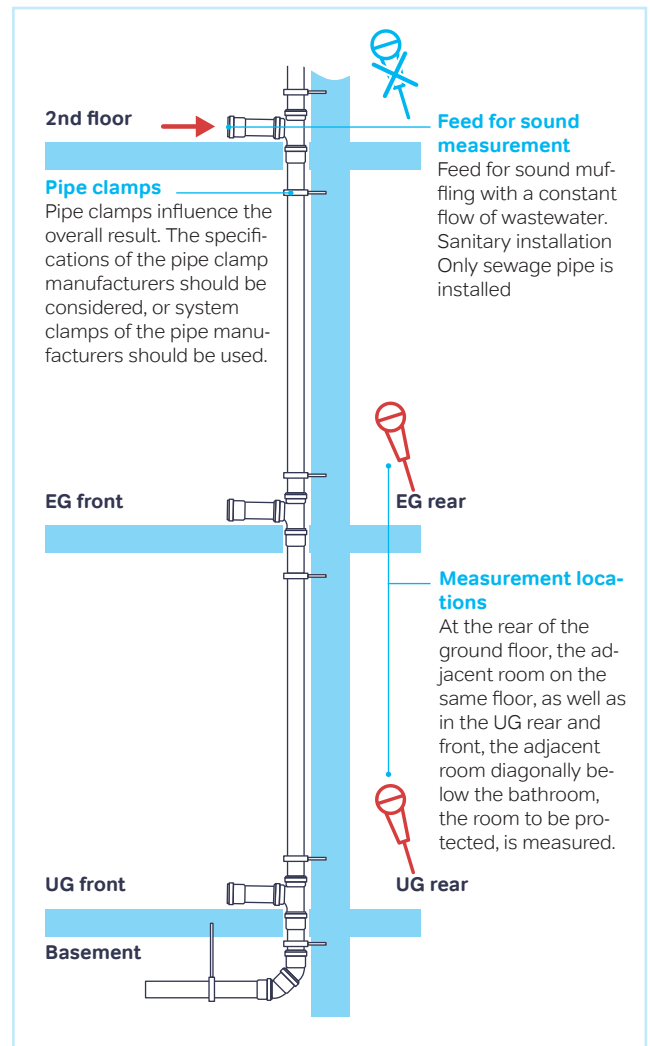
Figure 45: Measurement setup according to DIN EN 14366
