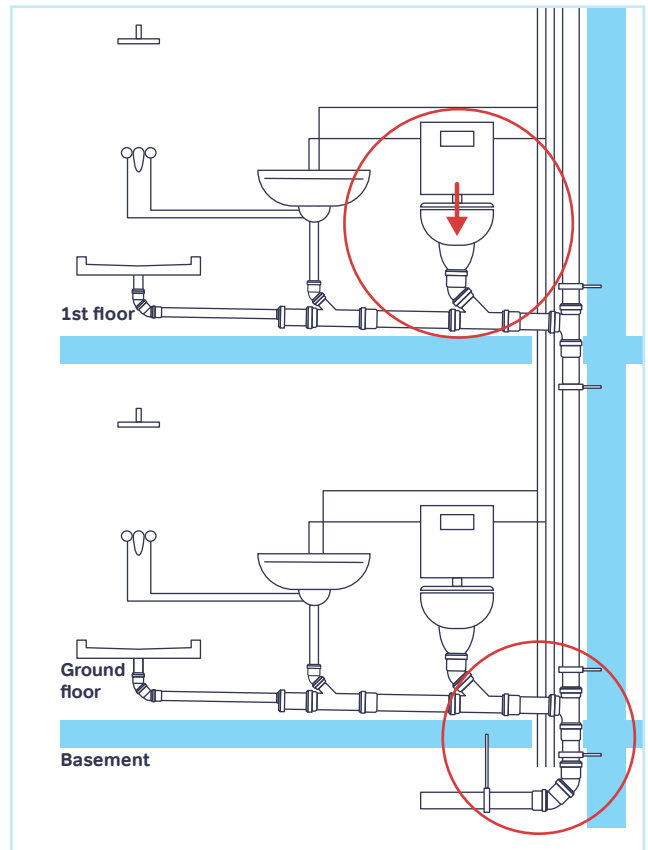
Figure 48: Main sound sources according to DIN 4109
