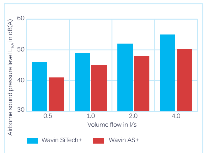
Figure 46: Influence of the pipe quality on the airborne sound pressure level
