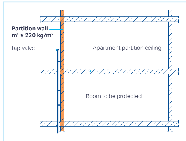
Figure 27: Arrangement of fittings of fitting group I
