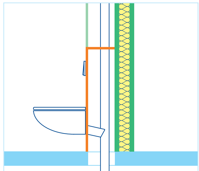
Figure 32: Curtain wall installation in front of a drywall panel (based on source 8)
