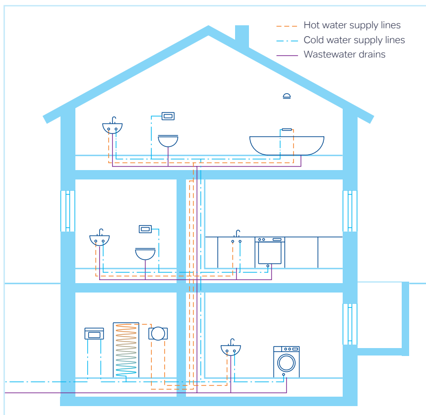
Figure 15: Supply and disposal lines in a building
