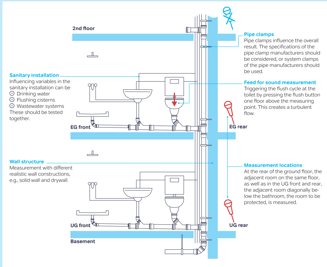
Figure 9: Representative setup for a measurement under real conditions.
