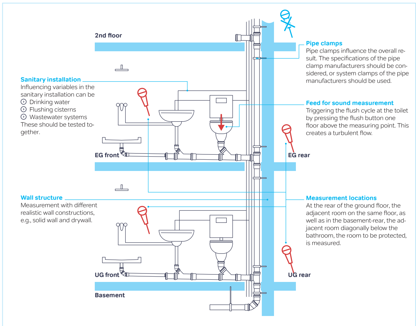
Figure 47: Representative setup for a measurement under real conditions.
