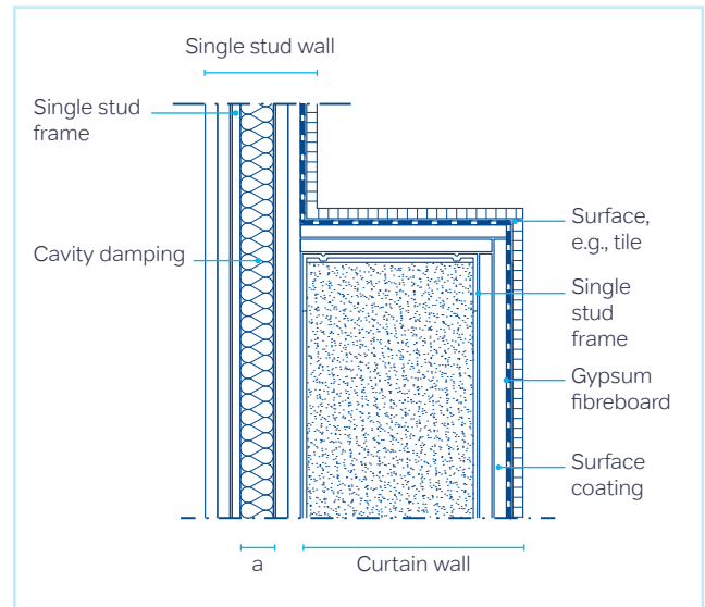
Figure 29: Single stud wall with additional curtain wall installation
