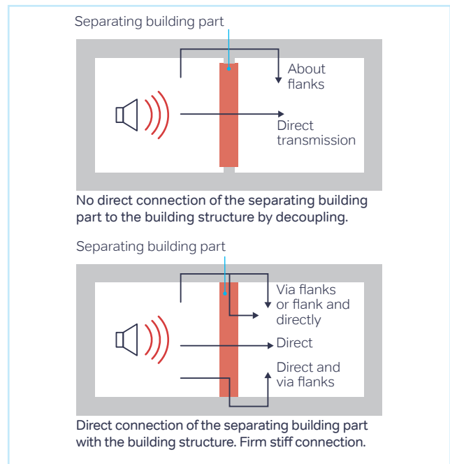
Figure 7: Information on the possible transmission paths for different building parts
