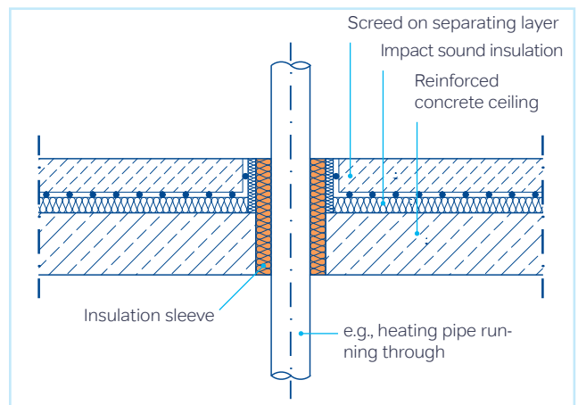
Figure 19: Pipe feedthrough without sound bridge
