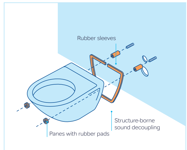
Figure 26: Design of a wall hung toilet system without sound bridges
