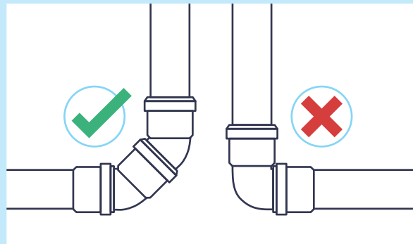
Figure 25: Installation situation with different bends
