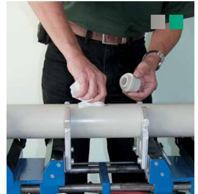
2. Clean. If you use the Stabi pipe, chamfer the edge of the drilled hole. Clean and degrease the weld-in saddle as well as the drilled hole.
