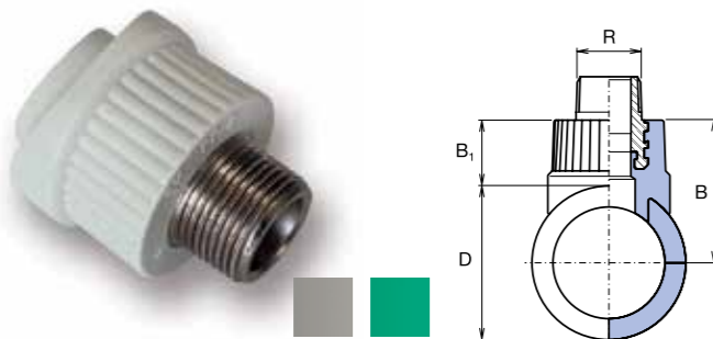
Weld-in saddle with metal thread male
