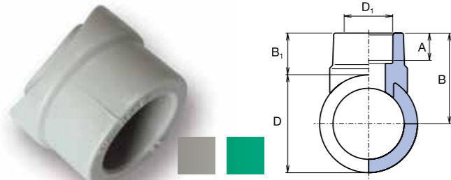
All-plastic weld-in saddle
