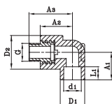
Underplaster Male Elbow
