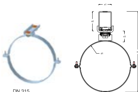
DN 315
