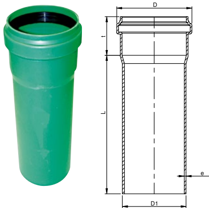
Green Connect 2000 – trubka s hrdlem
