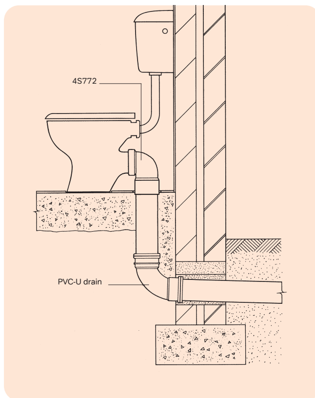
Figure 24: Connection to ground floor WC
