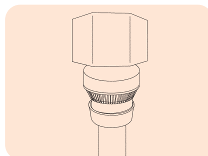
Figure 56: Installation of OsmaVent 40 – In areas of extreme temperatures
