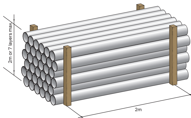
Figure 35: Storage of loose pipe on bearers
