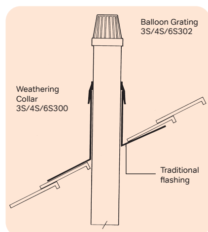
Figure 57: Installation of Weathering Collar
