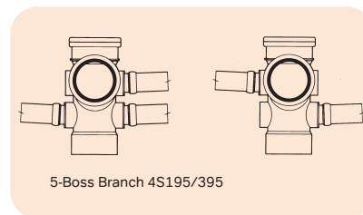
Figure 49: Connections NOT permitted
