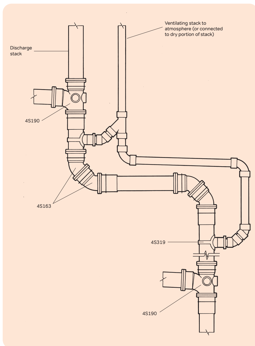
Figure 8: Ventilation stack to atmosphere
