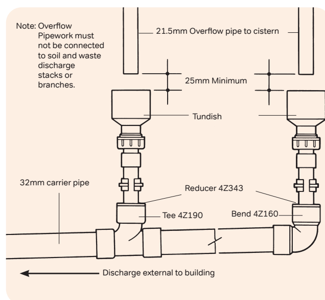
Figure 64: Typical Tundish – carrier pipe installation
