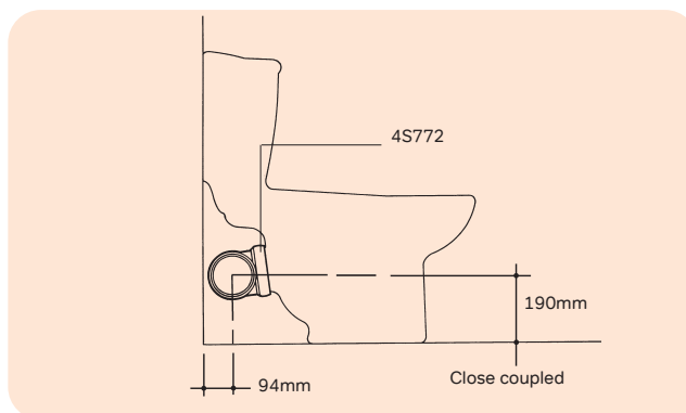
Figure 25: Alternative connection to WCs
