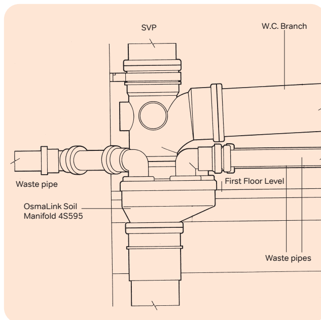
Figure 53: Typical OsmaLink Soil Manifold installation (side view)
