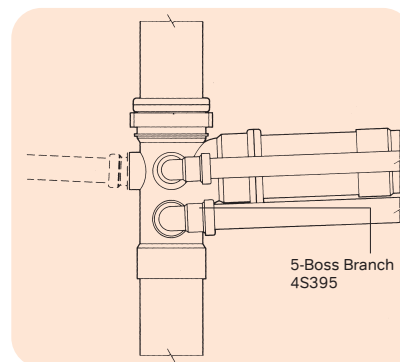
Figure 50: Connection of multiple wastes
