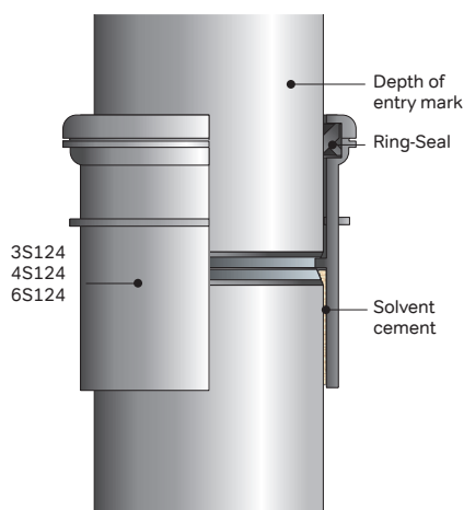
Figure 38: Solvent cement joint
