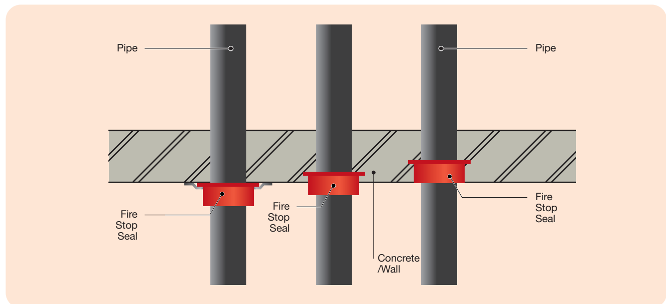
Figure 32: Fixing positions for Fire Stop Seals in concrete floor/masonry wall
