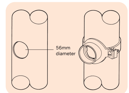
Figure 51: Connection of Strap Bosses
