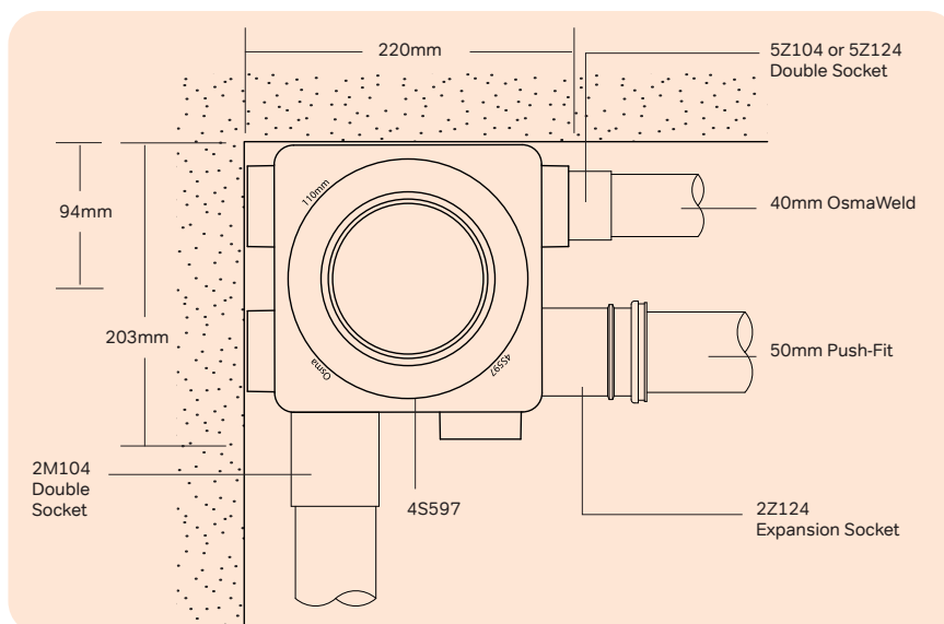
Figure 18: Typical Connections to 6 Boss Soil Manifold
