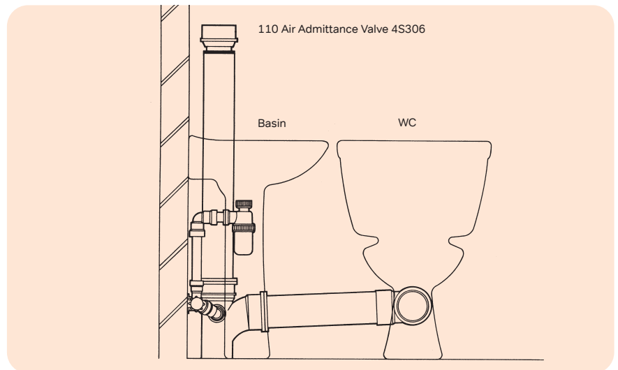
Figure 55: Vented stub stack
