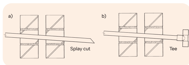
Figure 61: Terminating overflow pipe
