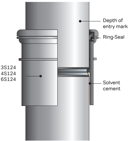
Figure 37: Ring-seal joint
