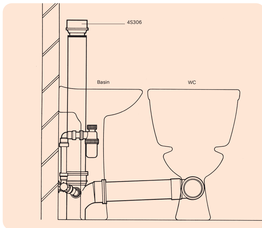
Figure 30: Vented stub stack
