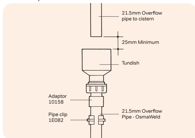
Figure 62: Tundish connection to 21.5mm Solvent Weld Overflow Pipe
