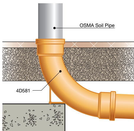
Figure 41: PVC-U drain socket (via 4D581)
