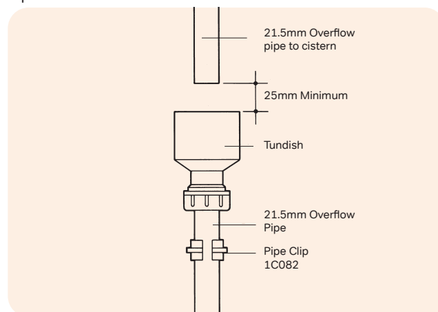
Figure 63: Tundish connection to 21.5mm Push-Fit Overflow Pipe
