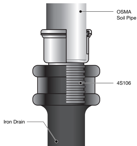
Figure 44: Cast iron drain socket
