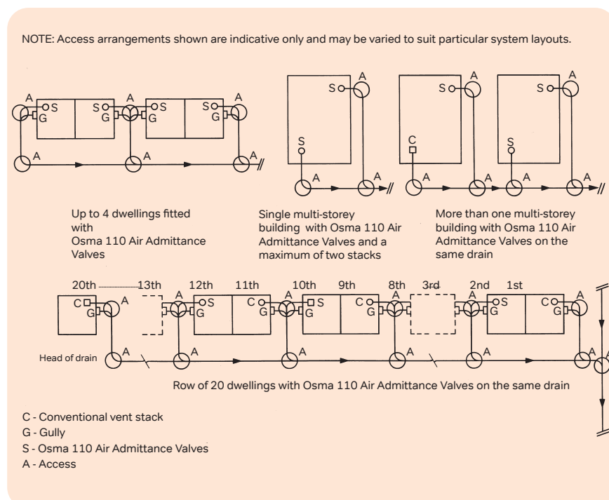
Figure 31: Examples of provisions for drain ventilation
