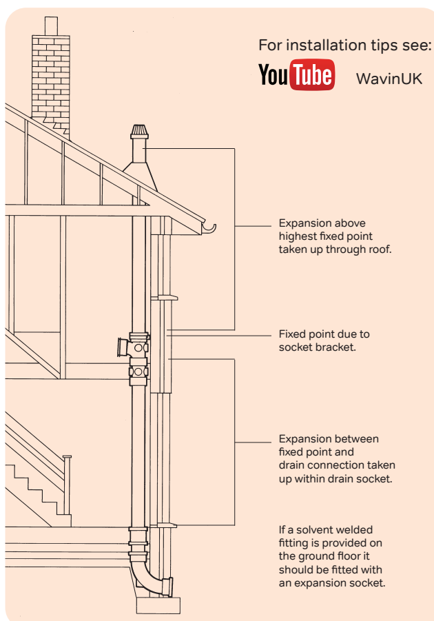
Figure 5: Thermal movement requirements for a Solvent Weld Soil system
