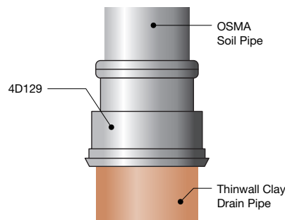
Figure 43: Thin-wall drain spigot
