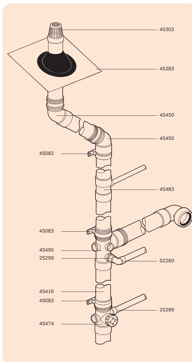
Figure 2: Typical stack assembly – Solvent Weld system
