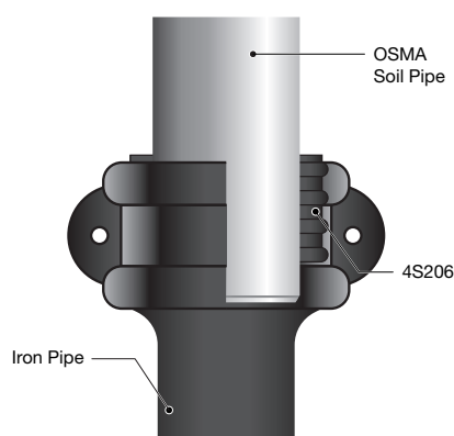
Figure 45: Cast iron soil socket
