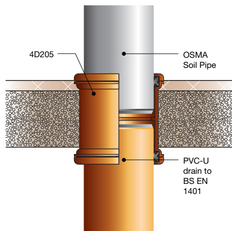
Figure 42: PVC-U drain spigot (via 4D205)
