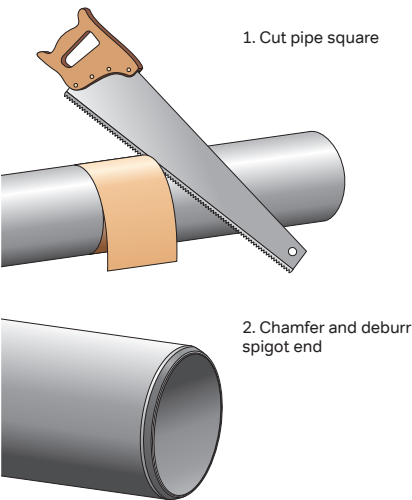
Figure 36: Pipe preparation
