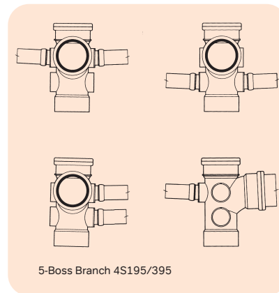
Figure 48: Permitted connections
