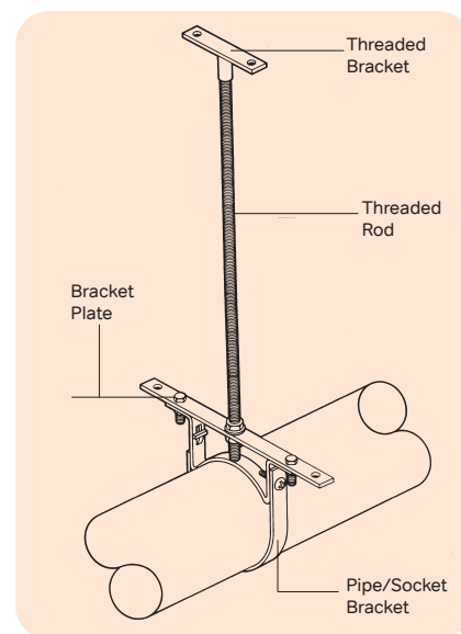
Figure 40: Suspended Bracketing (intermediate pipe support)
