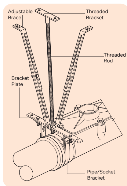
Figure 39: Suspended Bracketing (socket support)
