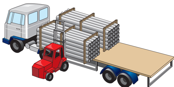
Figure 33: Unloading of block bundles
