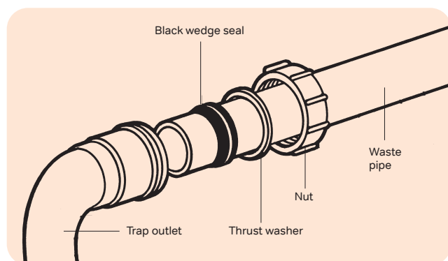
Figure 60: Connection to V-joint trap outlet
