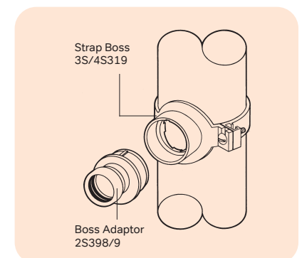
Figure 52: Fitting Boss Socket Adaptor
