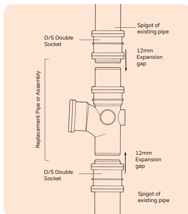
Figure 65: Incorporating a fitting
