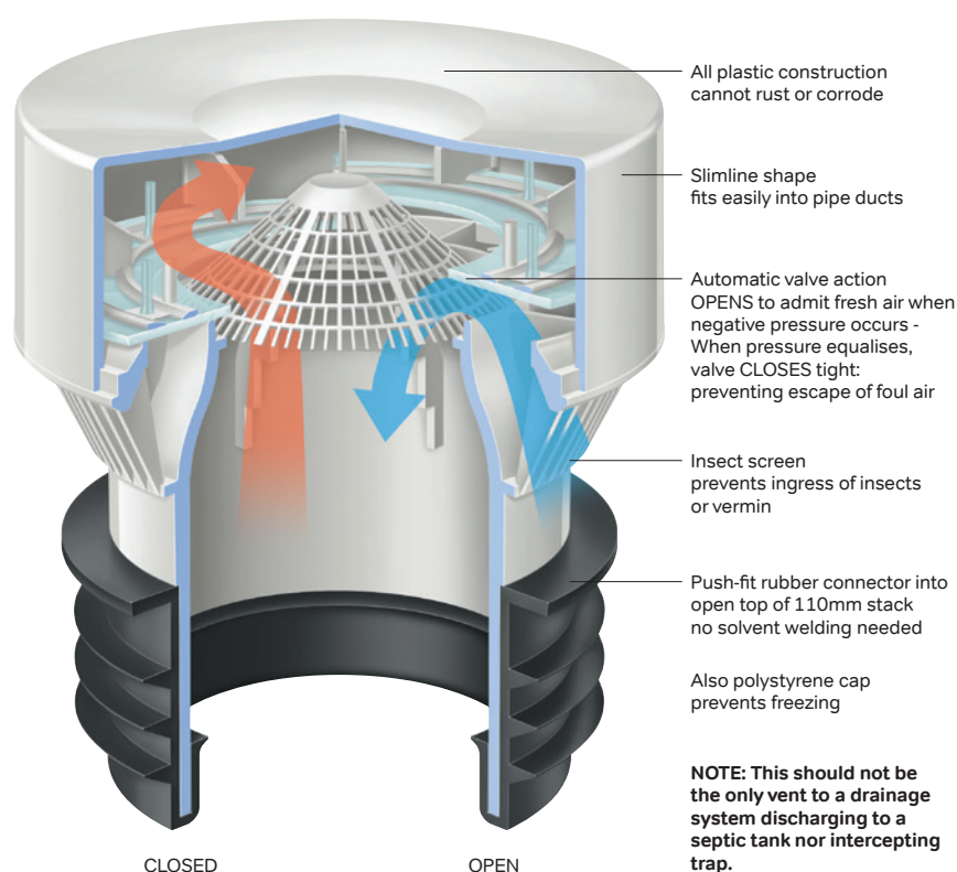
Figure 29: Valve operation
