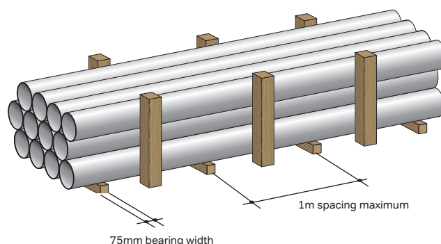
Figure 35: Storage of loose pipe on bearers
