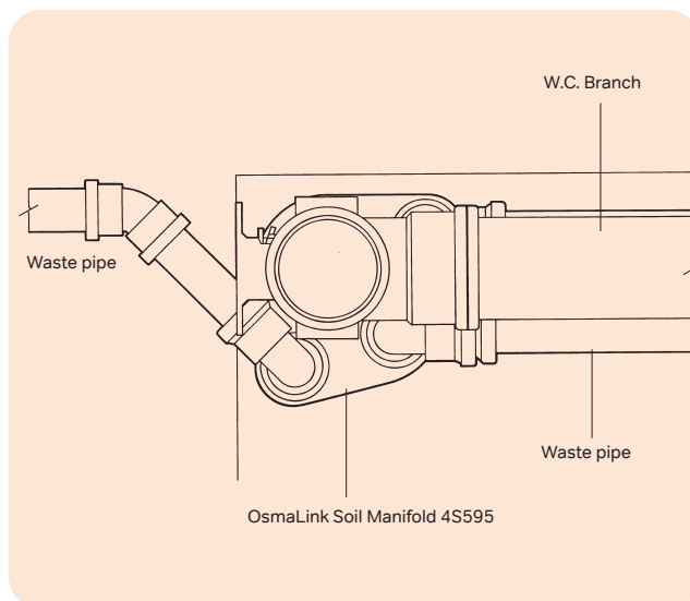
Figure 54: Typical OsmaLink Soil Manifold installation (plan view)
