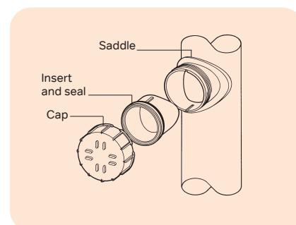
Figure 46: Access Saddle
